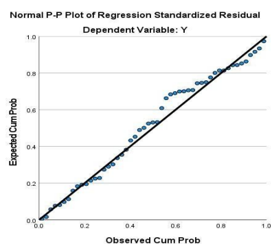
Gambar 4 3. Grafik Normal P-P Plot
